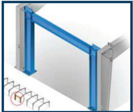
Portal Bracing
